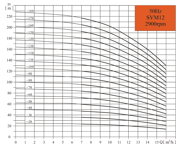
Performance curves
